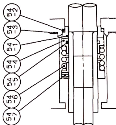
CLOSE-UP VIEW OF MECHANICAL SEAL
